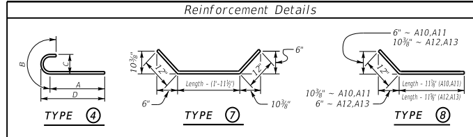
Reinforcement Details
